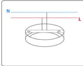
2. Fix the power supply at the bottom of the lamp, and connect the two power cables to the L/N of the 220V power cable.
